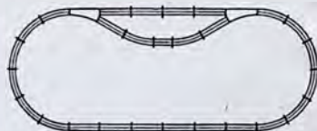
No. 3—40" x 100"—Requires 14 Curve, 12 Straight, one ½ straight track and 1 Pr. of Switches.
