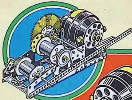
Two-drum Hoist with P56G 110 volt motor.
