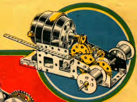
Three-step worm drive with P56G 110 volt motor.
