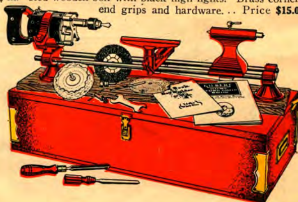
No. 795 MOTOR DRIVEN HOME WORKSHOP. Complete craftsman's set for home or commercial use. Portable type, standard equipment, practical and efficient. This lathe is turned by a powerful 110 volt motor with interchangeable parts for turning, spinning, grinding, polishing, buffing, etc. Motor has pistol grip and when detached from motor is converted into a powerful electric drill. Assortment of accessory units and instructions. Size 30 in. long x 8 in. wide x 8\frac{1}{4} in. deep. Individually packed in a large stained red wood cabinet with brass end grips and reinforced corners and lock. Price $35.00
