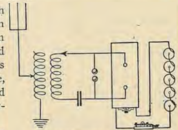
TUNED TRANSMITTING SET
